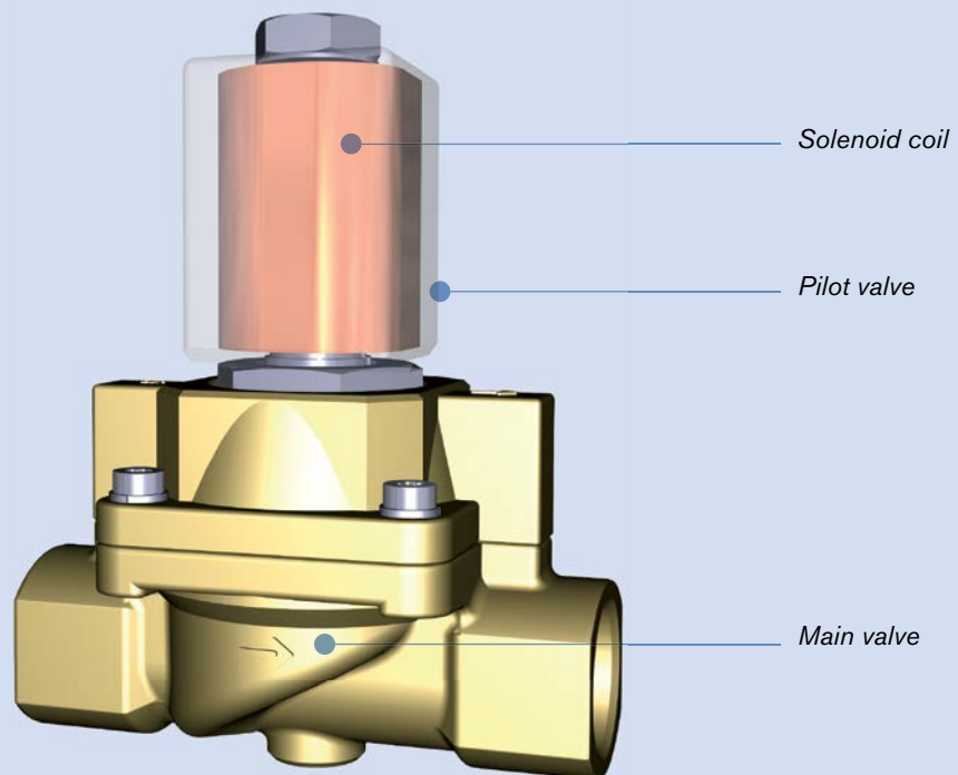
2/2-way servo-assisted piston valve type 0406
