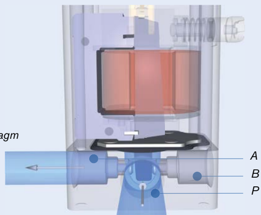
Distribution valve Energised
