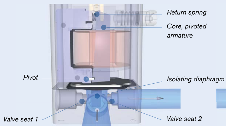
Distribution valve De-energised
