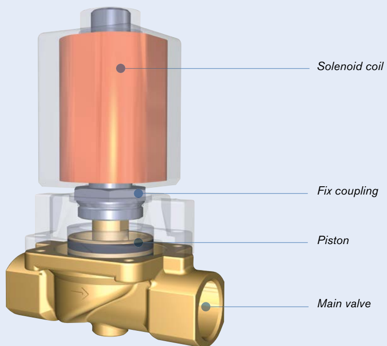
Servo-assisted piston valve, fixed coupled, type 407
